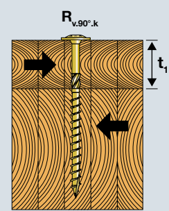
Shear Perpendicular (90°) to the Grain
