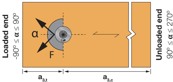
Laterally Loaded Screws - Minimum spacing or end/edge distance
