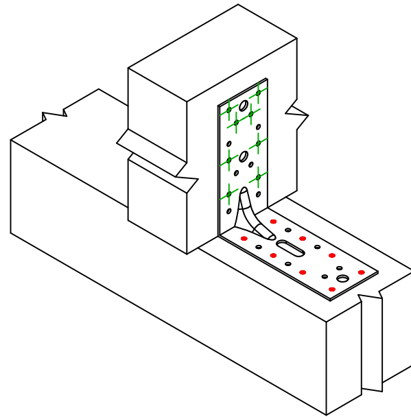
Installation for 1 bracket
