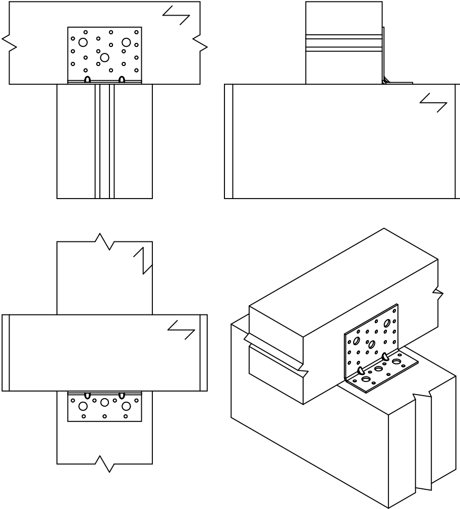
Installation for 1 bracket
