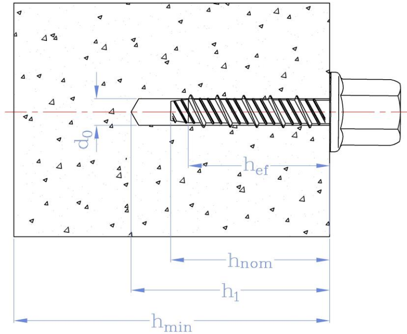
Drawing A2. Installed condition for anchors CLR6-D, CLR6-U, CLR6-F, CLR6-E, CLR6-C, CLR6-G, CLR6-I, CLR6-Q and CLR6-V.
