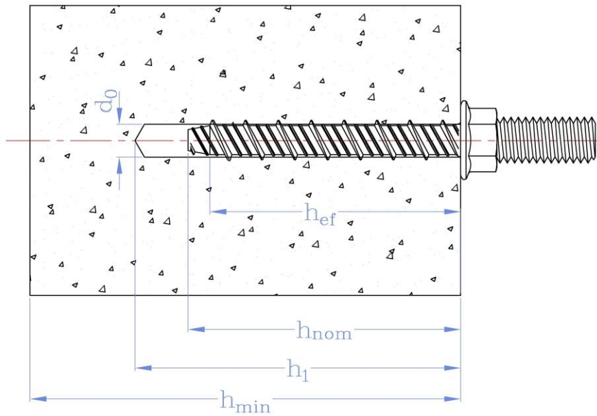
Drawing A3. Installed condition for anchors CLR6-D, CLR6-U, CLR6-F, CLR6-E, CLR6-C, CLR6-G, CLR6-I, CLR6-Q and CLR6-V.
